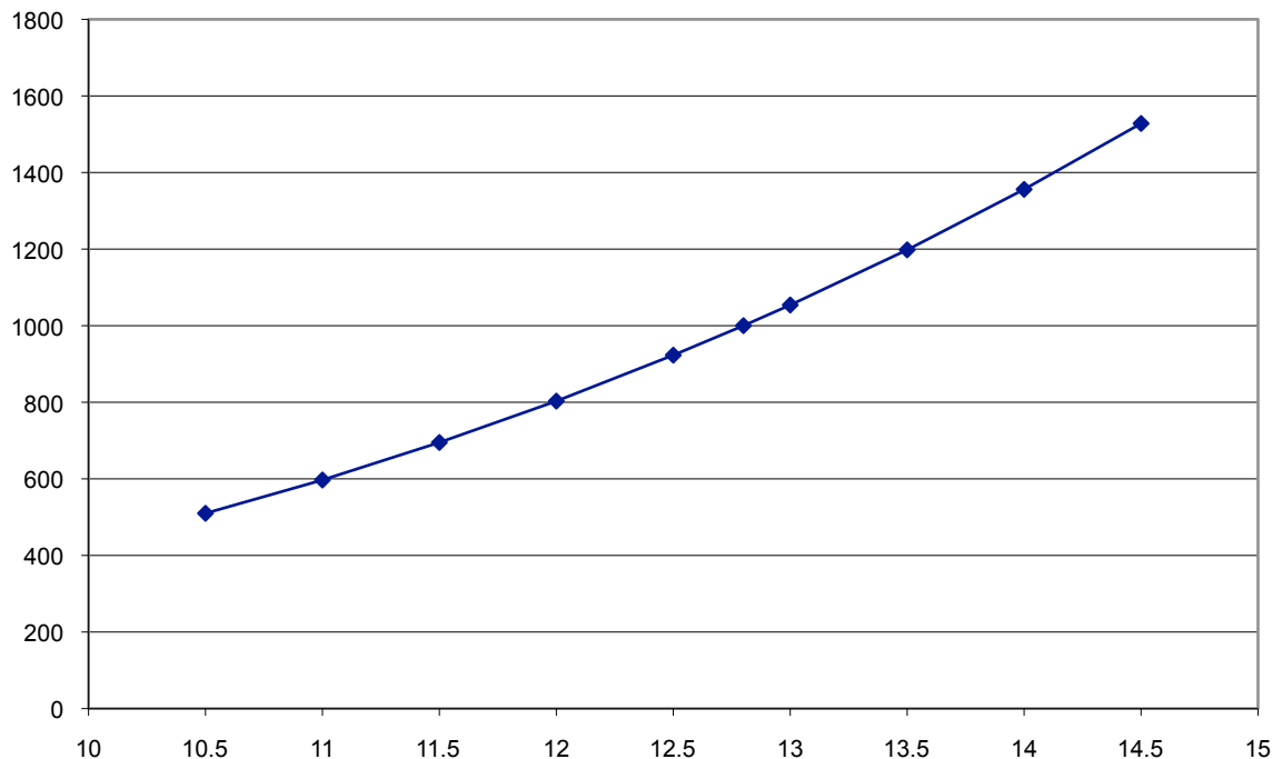
H4 lumens vs voltage at the bulb
